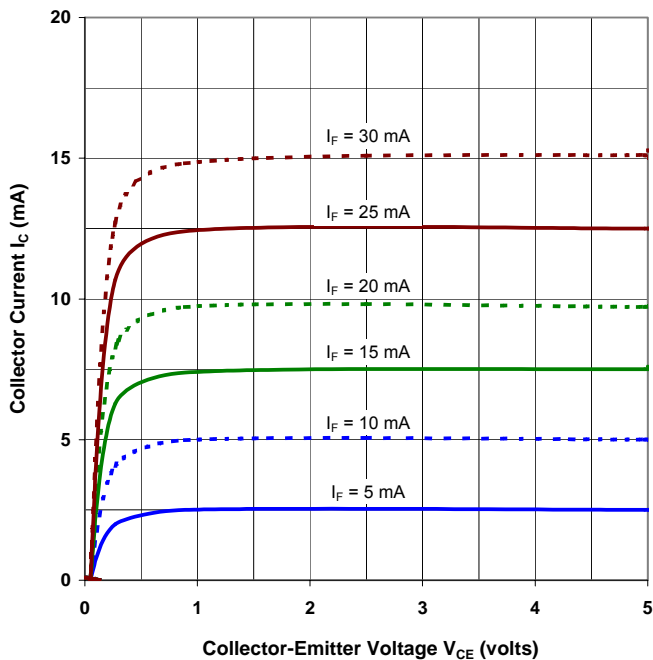
OPB202 - Collector Current vs Collector-Emitter Voltage
