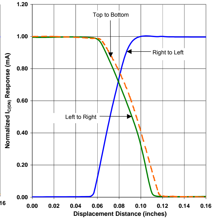
OPB202 - Flag Next to Sensor
