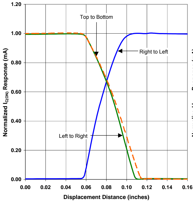
OPB202 - Flag Next to Emitter
