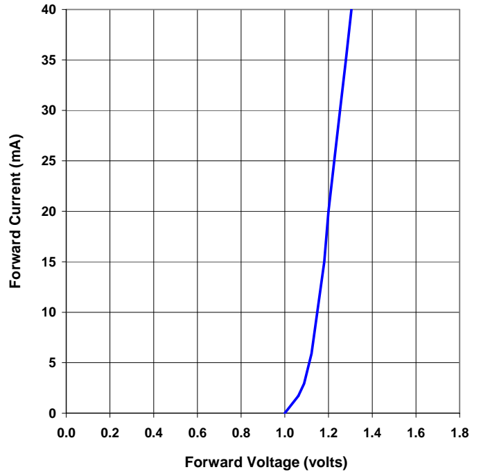
OPB202 - Forward Current vs Forward Voltage
