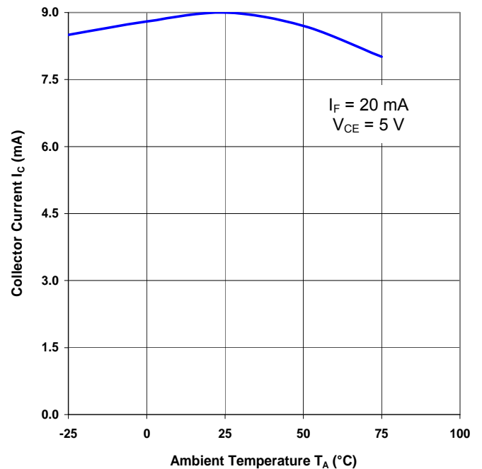
OPB202 - Collector Current vs Ambient Temperature
