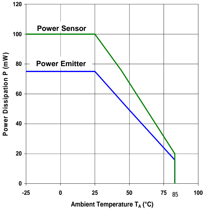
OPB202 - Power Dissipation vs Ambient Temperature
